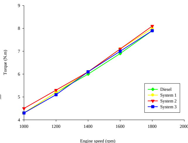
Figure 1. Engine torque at varying engine speed of the water microemulsified diesel at low load
