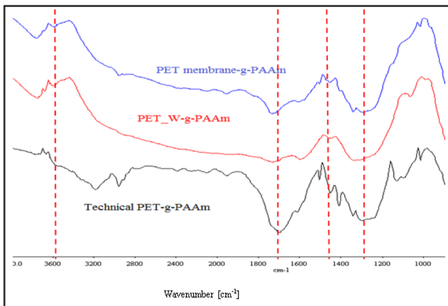
Figure 6. FTIR spectra of modified PET membrane, PET_W and technical PET.
