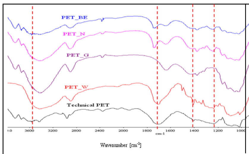
Figure 2. FTIR spectra of unmodified PET textiles.
