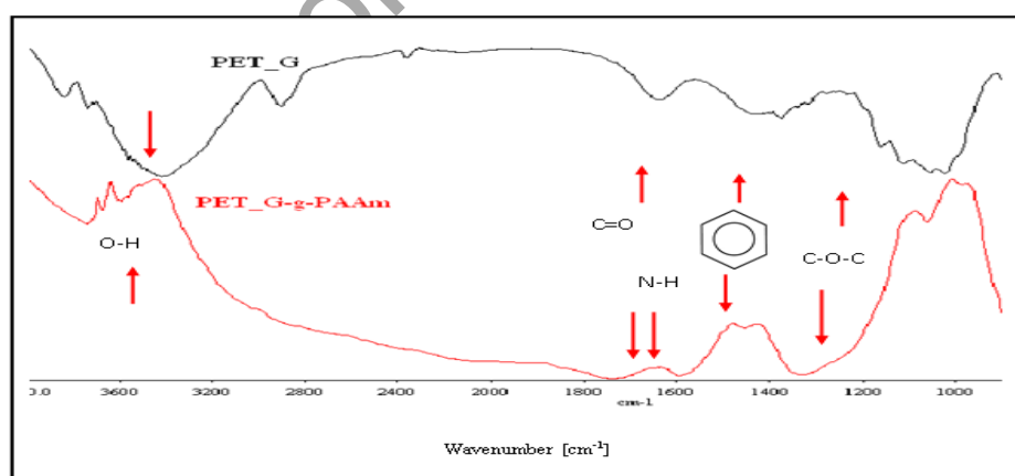
Figure 5. FTIR spectra of unmodified and grafted PET textiles (PET_G)
