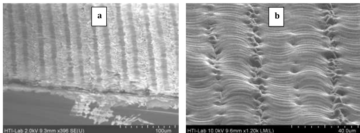
Figure 7. SEM image of one-dimensional laser-scanned annealing at 25- \mu m period under different magnification, (a) under magnification 396, and (b) under magnification 1.2k
