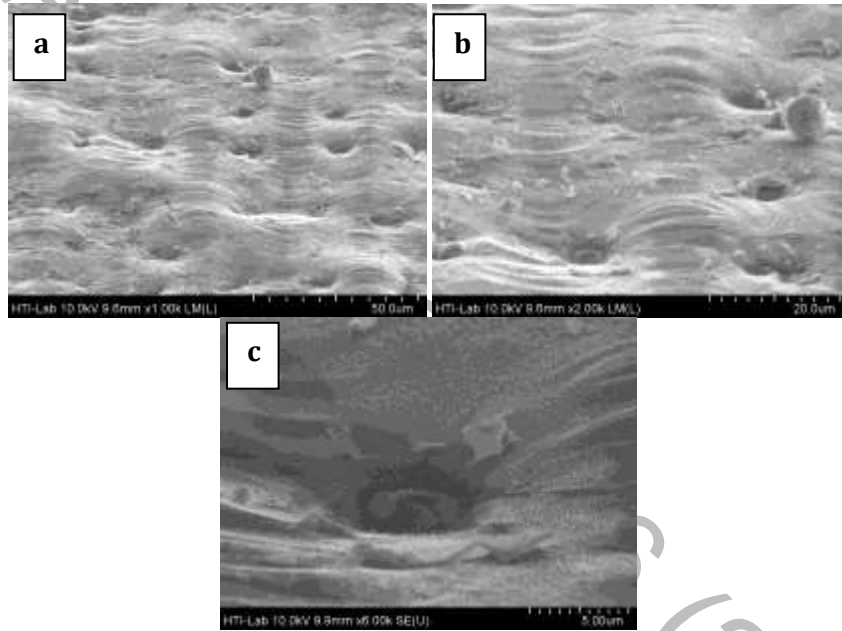
Figure 10. SEM pictures of two-dimensional laser-scanned surfaces at 25- \mu m period under different magnification, (a) under magnification 1k, (b) under magnification 2k, and (c) under magnification 6k
