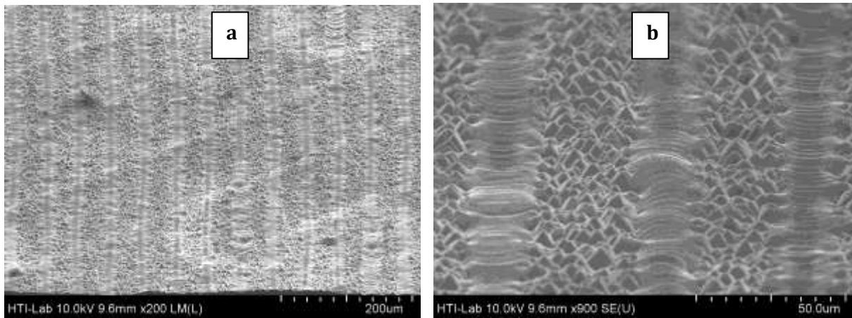
Figure 5. SEM image of one-dimensional laser-scanned annealing at 50- \mu\text{m} period under different magnification, (a) under magnification 200, and (b) under magnification 900
