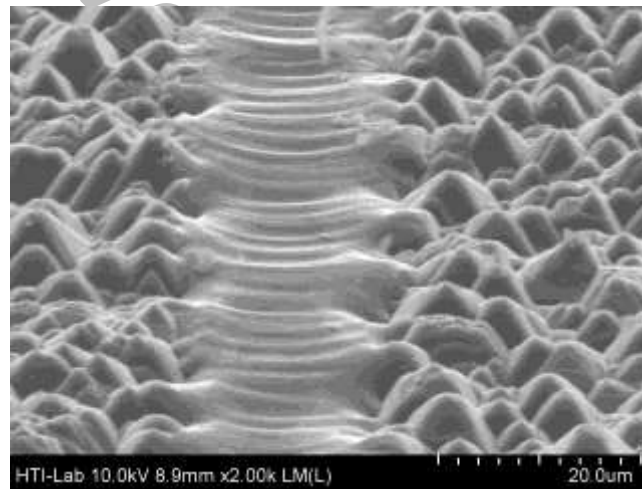
Figure 6. High resolution SEM pictures of one-dimensional laser-scanned surfaces at 50- \mu\text{m} period
