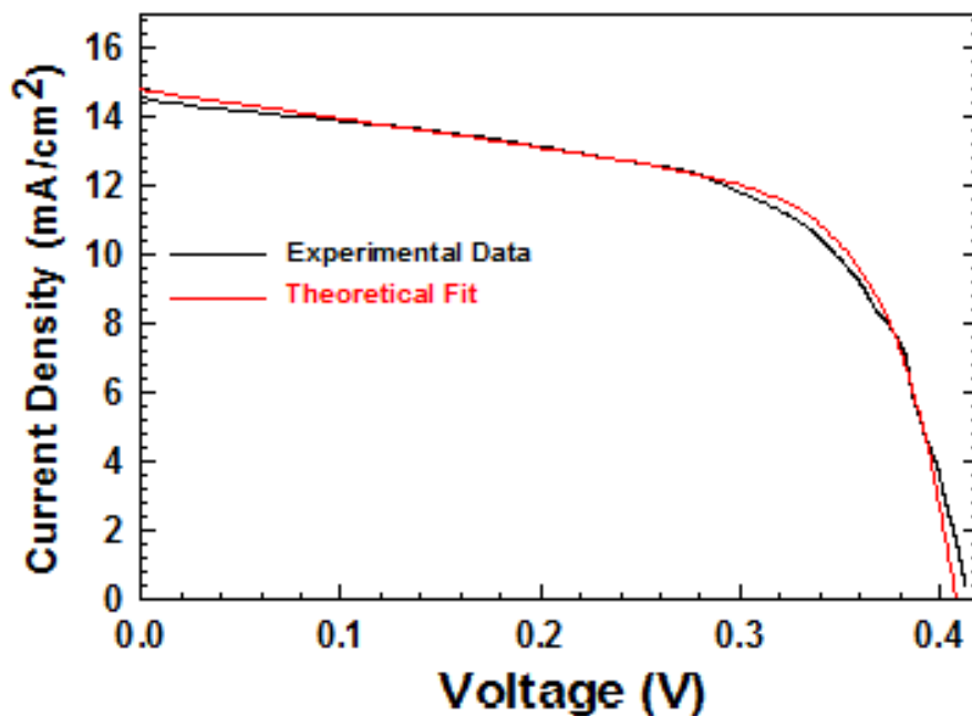
Figure 12. Comparison between experimental data and simulation data with the best fit of the data. Parameter conditions; Lifetime= 0.02 \mu sec, Shunt resistant= 50 \Omega , Doping concentration= 2.87 \times 10^{16} , Reflectance= 40%, Emitter resistant= 0.05 \Omega
