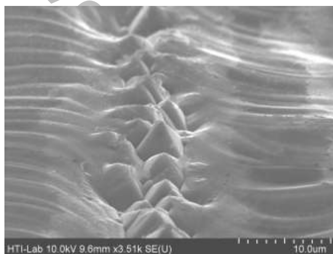
Figure 8. High resolution SEM pictures of one-dimensional laser-scanned surfaces at 25- \mu m period
