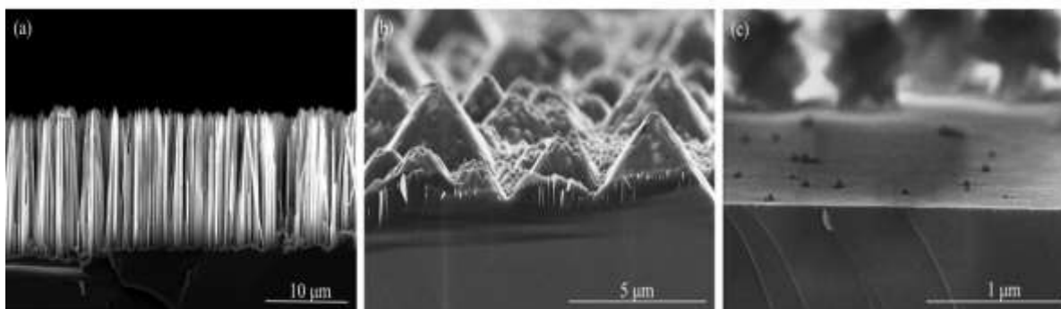
Figure 1. Cross-sectional view of (a) Si nanopillars (b) Si micropylramids and (c) polished Si profiles
