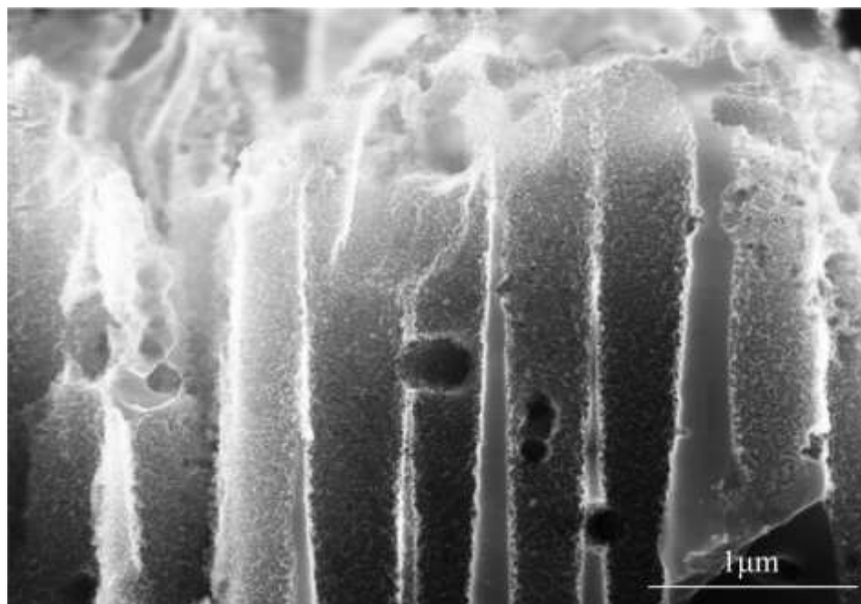
Figure 4. High magnification FE-SEM image of surface morphology of Si nanopillars. Etching was conducted in 0.55 M \text{H}_2\text{O}_2 for 40 minutes
