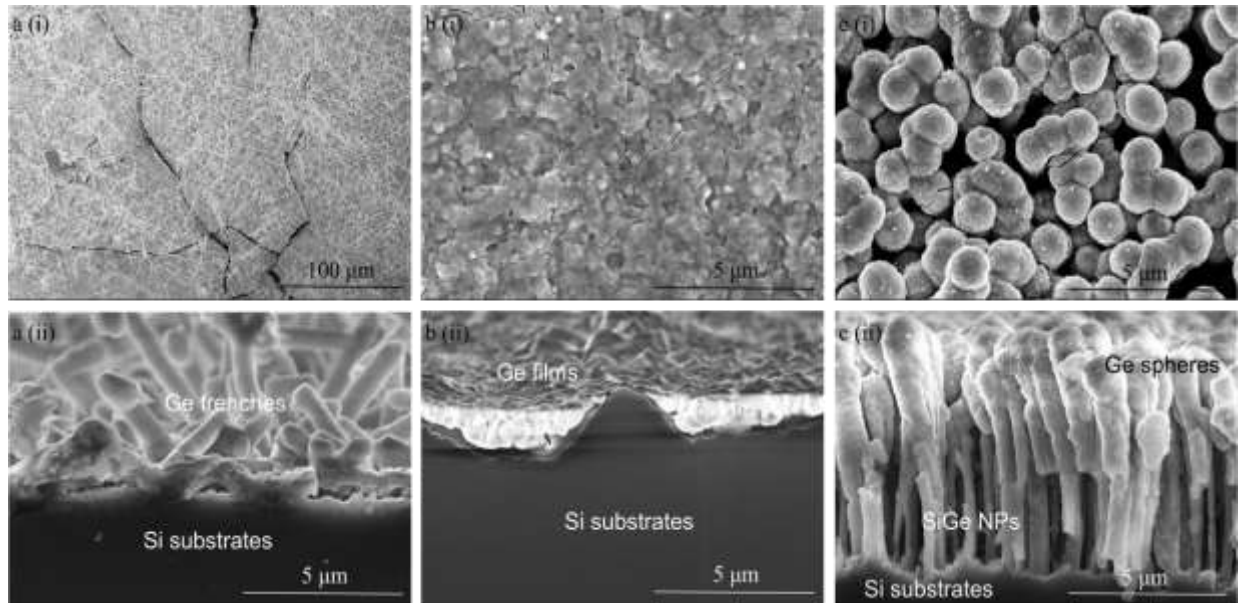
Figure 8. Surface and cross-sectional views of Ge deposited on (a) polished Si, (b) Si micropylamids and (c) Si nanopillars. Formations of cracks are visible for Ge deposited on polished Si and Si micropylamids.
