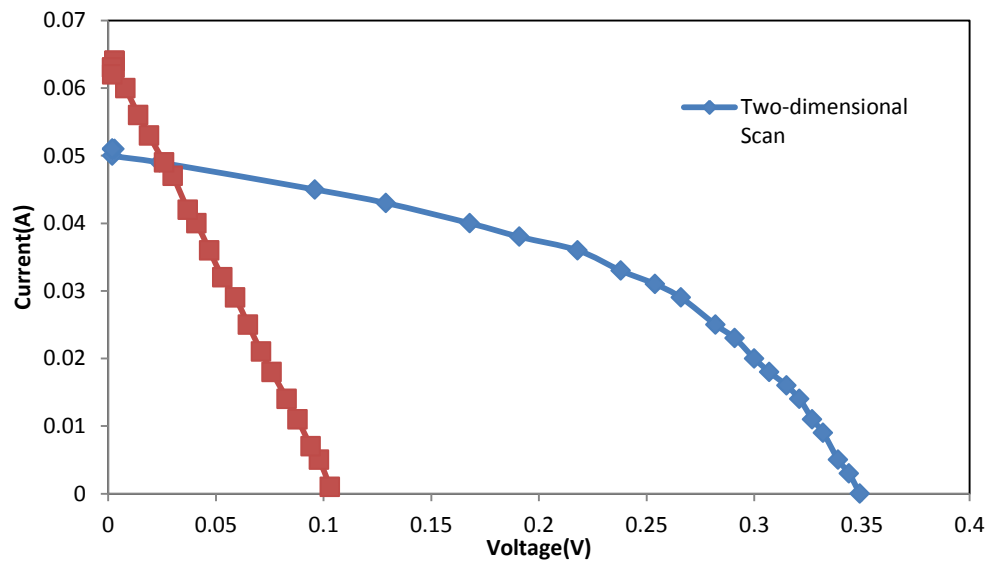
Figure 11. LIV data for one-dimensional and two-dimensional laser annealing scan solar cell
