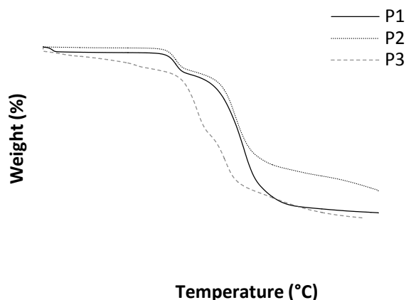
Figure 6. The TGA thermogram of P1 , P2 and P3 .
