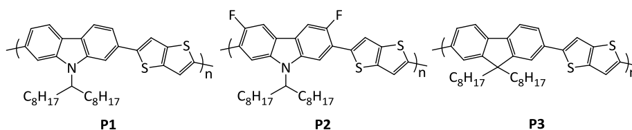
Figure 1. Structure of copolymers P1 , P2 and P3 .
