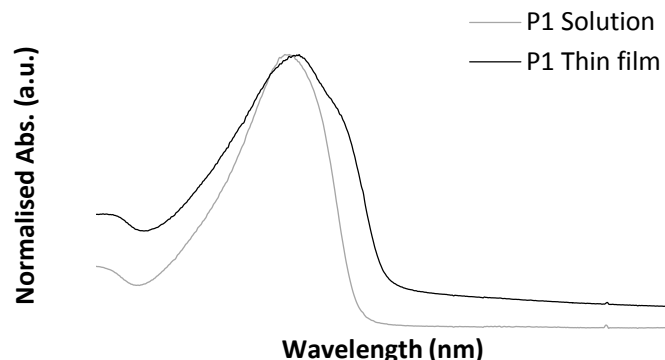
Figure 2. Normalised UV-Vis spectra of P1 in chloroform solution (grey line) and a thin film (black line).
