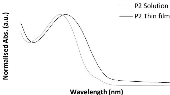
Figure 3. Normalised UV-Vis spectra of P2 in chloroform (grey line) and a thin film (black line).
