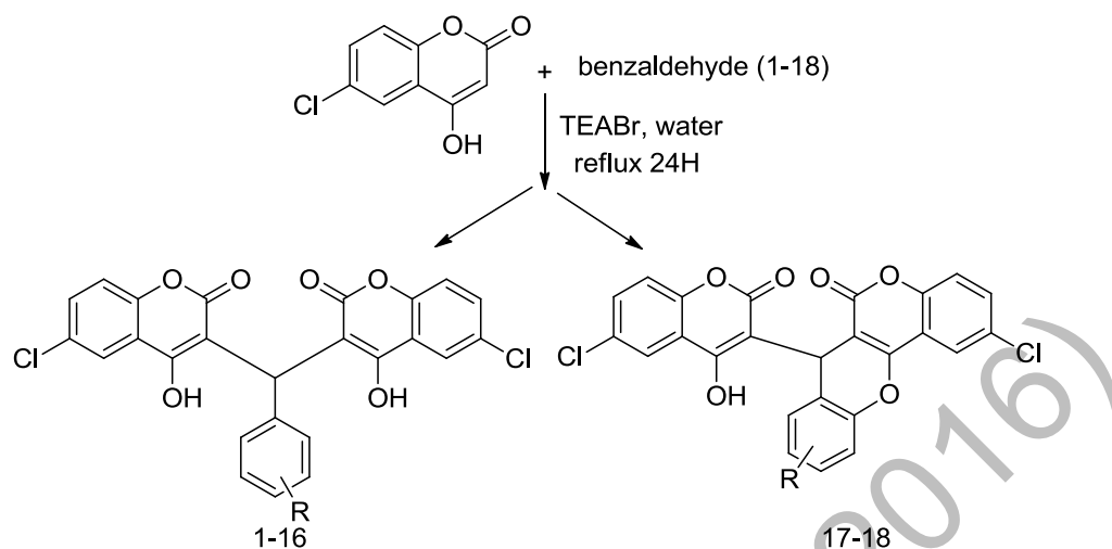
Scheme 1. Synthesis of biscoumarin (1-16) and benzopyrano dicoumarin derivatives (17-18)
