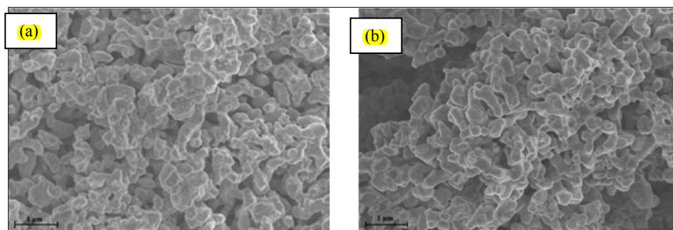
Figure 3. SEM micrographs of (a) EG900 powder and (b) AC900 powder
