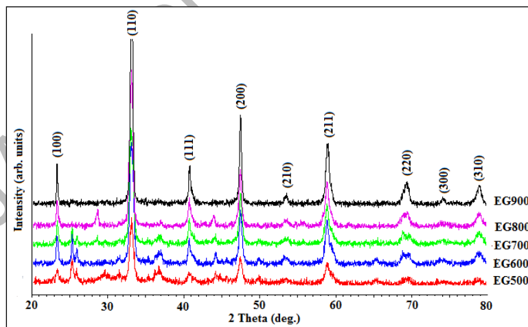
Figure 1. XRD patterns of the powders after calcined at various temperatures prepared using ethylene glycol (EG) as a surfactant
