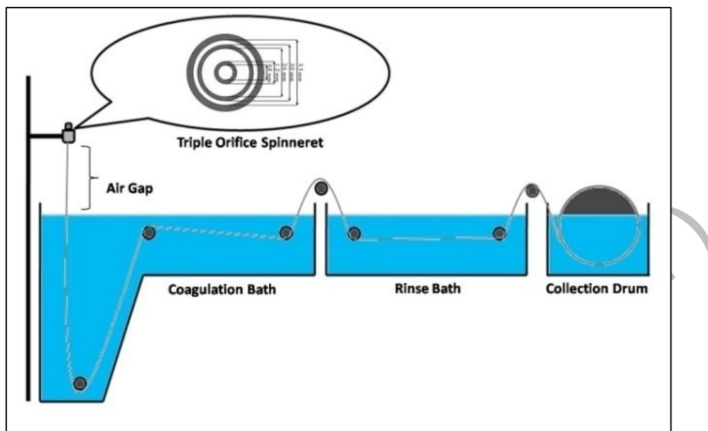
Figure 1. Dual layer hollow fiber spinning method
