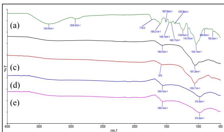
Figure 4. FTIR spectrum of (a) raw-PKS (b) 10%AC/K (c) 15%AC/K (d) 20%AC/K (e) 25%AC/K
