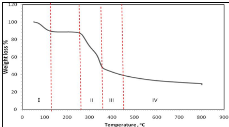
Figure 3. TGA curve of raw PKS
