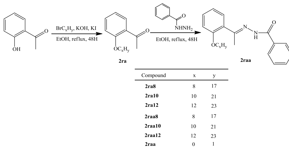
Scheme 1. Synthesis of hydrazone Schiff base compound and its derivatives
