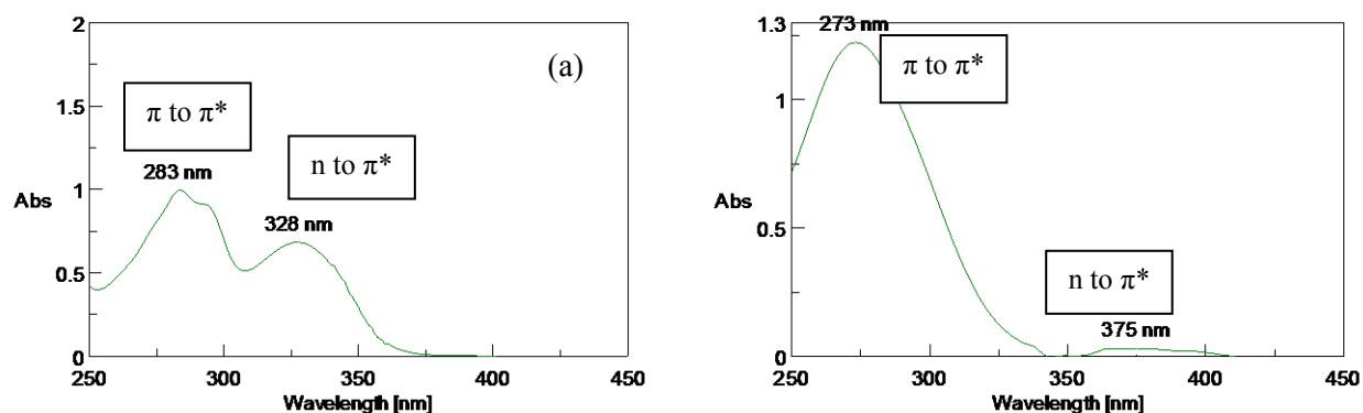
Figure 3. Electronic spectra of (a) parent compound ( 2raa ), (b) derivative of Schiff base compound ( 2raa8 )
