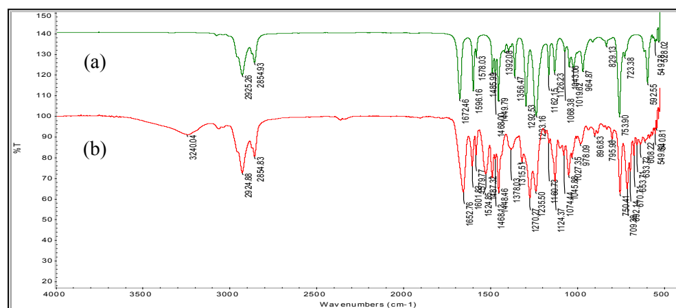
Figure 2. Infrared spectra of (a) etherified ketone, 2ra8 and (b) derivatives of Schiff base, 2raa8
