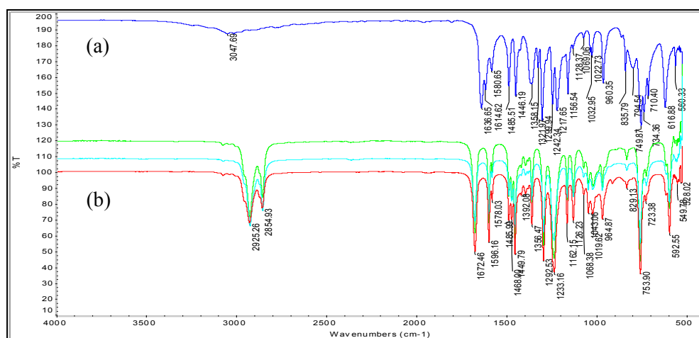
Figure 1. Infrared spectra of (a)starting material, 2-hydroxyacetophenone, (b)etherified 2-hydroxyacetophenone, 2ra8 – 2ra12
