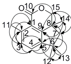
Figure 2. HMBC correlation of 10-Oxodehydrodihydrobotrydial ( 1 )
