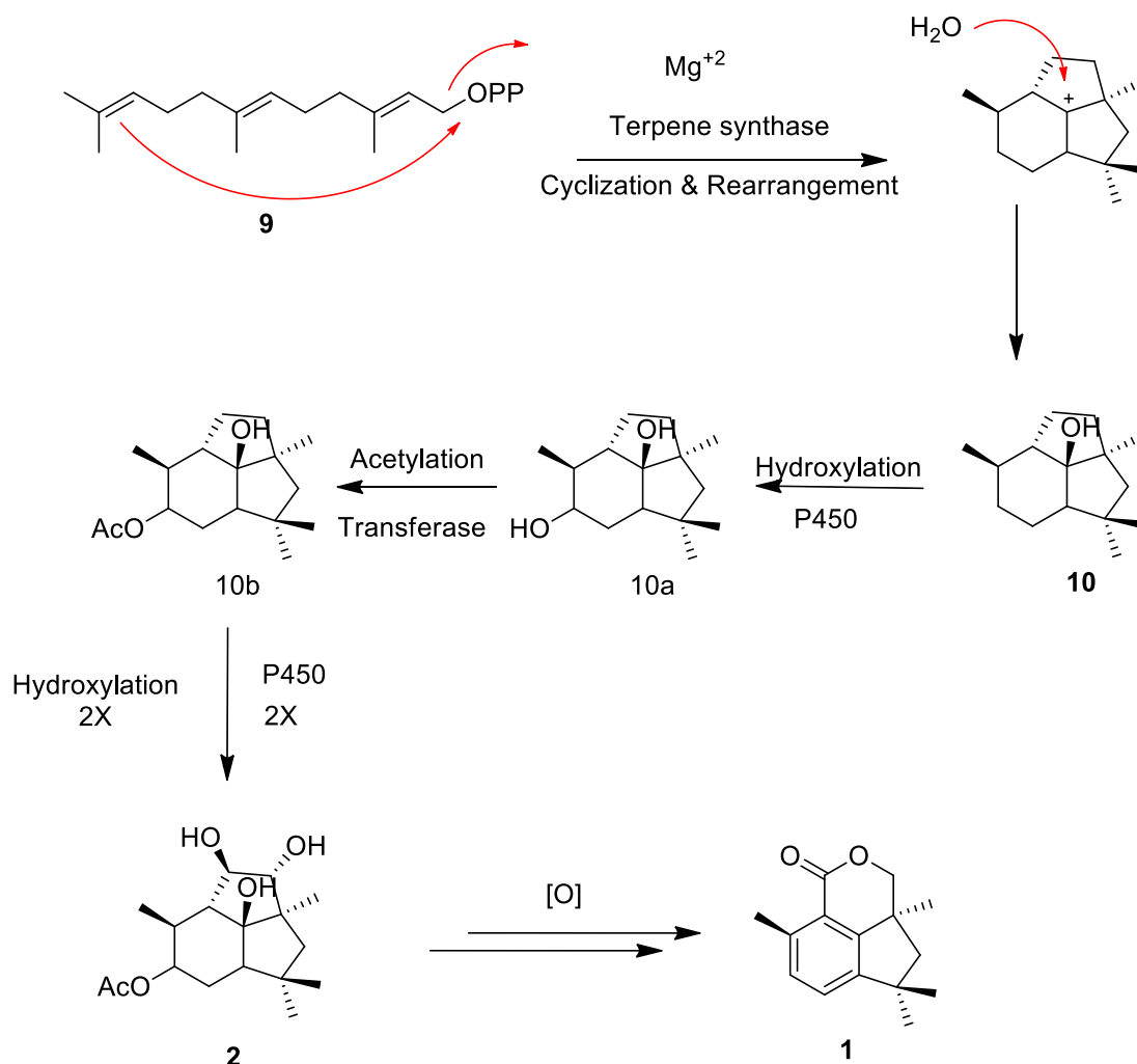
Figure 4 Proposed biosynthetic pathways of Botryane;
