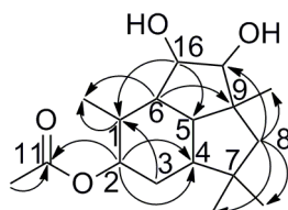
Figure 3. HMBC correlation of 4β-Acetoxy-9β,10β,15α-trihydroxybotrydial ( 2 )
