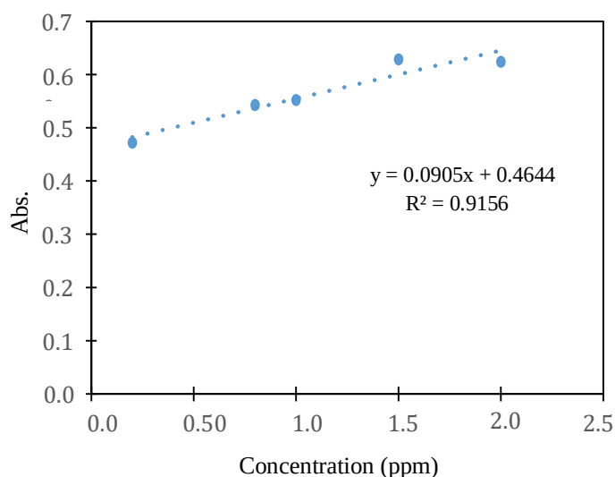
Figure 6. Calibration curve of absorbance against concentration of DA
