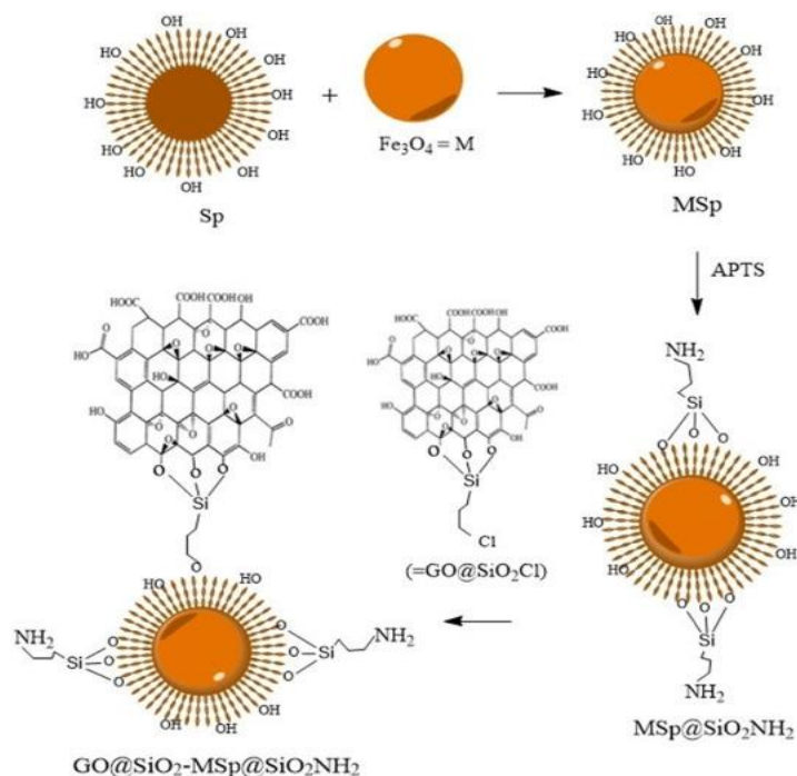
Figure 2. Schematic routes for the preparation of GO@SiO 2 -MSp@SiO 2 NH 2 [79]
