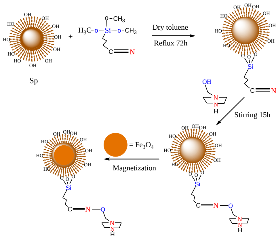
Figure 1. Schematic routes for the preparation of 1-(2-hydroxyethyl) piperazine-functionalized magnetic-Sp (MNPs-Sp-HEP)
