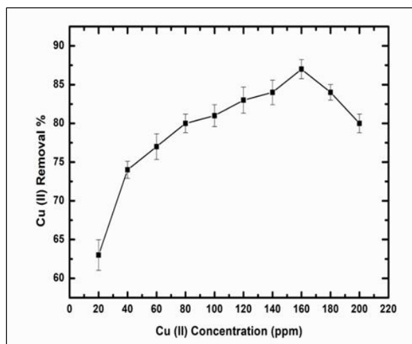
Figure 2. Removal efficiency of Cu(II) from aqueous solution using fixed amount of PVBC at different Cu(II) concentrations (ppm). Extraction conditions: 6 mg of adsorbent dose, temperature 22 °C, batch volume 5 mL, time 3 hours, and pH 4. Data are mean of three independent determinations \pm standard deviation
