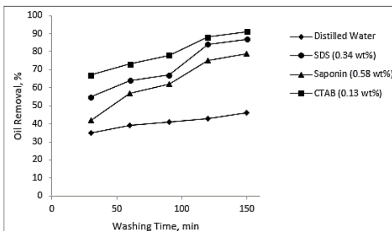
Figure 4. Oil removal percentage versus washing time.
