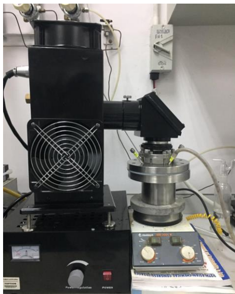
Figure 1. Photoreactor set up for the photocatalytic \text{H}_2 generation measurements
