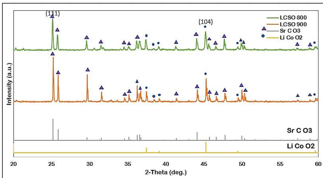
Figure 4. XRD spectrum obtained by this research
