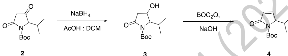
Scheme 3. The reduction and elimination reaction of the functional group at the C-4 position of compound 2
